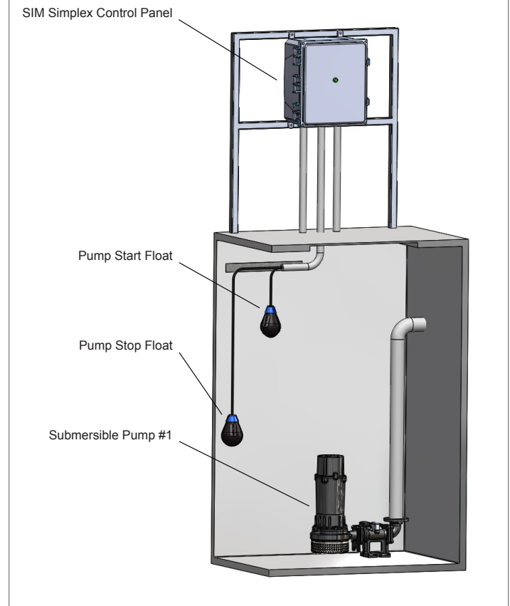
Typical Installation of SIM Simplex Control Panel
